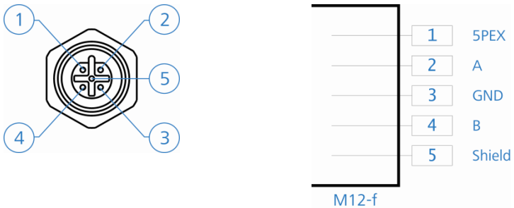
Figure 11 : Connection diagram LDM301P Profibus-OUT
