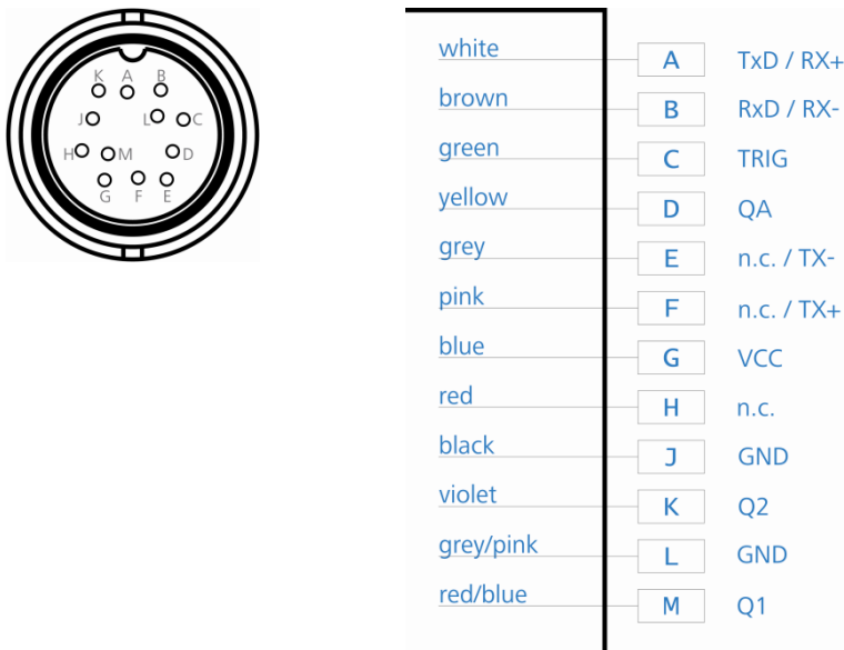
Figure 8 : Connection drawing of the main connector
