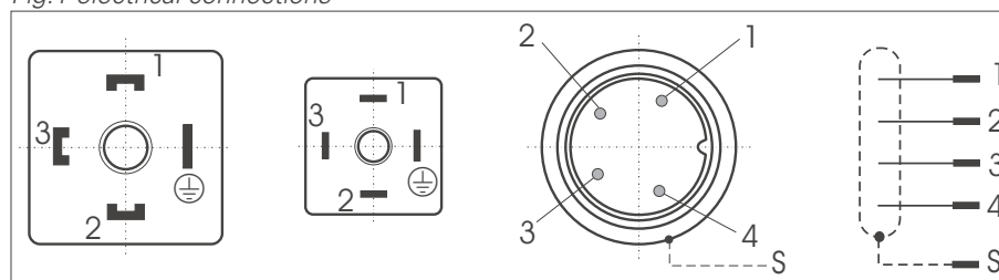
Fig.1 electrical connections
